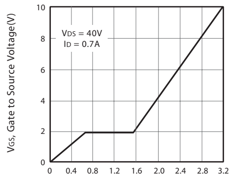
Figure 10. Gate Charge
